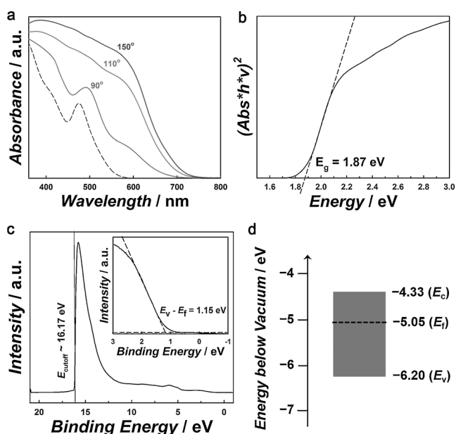
Figure 3. a) UV/Vis spectra of Ag-Bi-I thin-films as a function of annealing temperature. b) Tauc plot of AgBi 2 I 7 from the UV/Vis spectroscopy to determine E_g under the assumption of a direct band gap. c) UPS spectrum in high binding-energy region of AgBi 2 I 7 film annealed at 150 °C to determine the E_{\text{cutoff}} level. Inset: linear extrapolation in the low-binding-energy region for the value of ( E_v - E_f ). d) Energy band diagram of AgBi 2 I 7 film calculated from the Tauc plot and UPS results.
