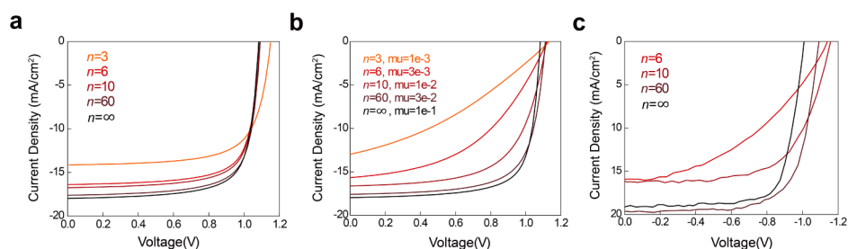
Figure 4. Comparison of J - V curves for different numbers of perovskite layers. (a) Simulation using experimental absorption spectra and band gaps, and mobility of 0.1 \text{ cm}^2 \text{ V}^{-1} \text{ s}^{-1} . (b) Simulation with radiative recombination of 5 \times 10^{-10} \text{ cm}^3 \text{ s}^{-1} and gradually decreasing mobility for lower n . Same trap density is used for all cases. Perovskite layer was estimated to be 200 nm thick. (c) Experimental curves.
