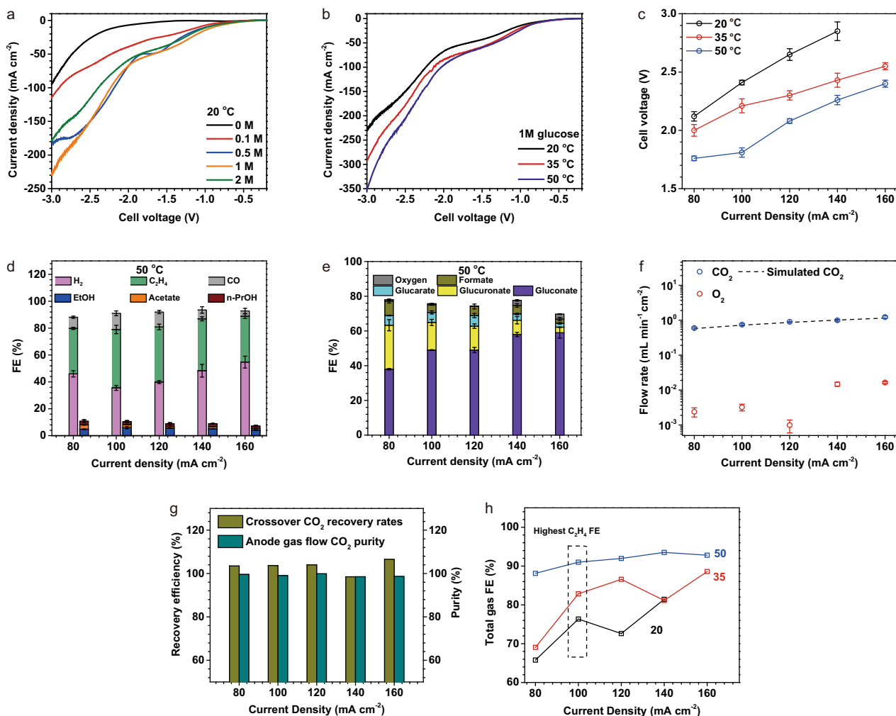
Fig. 3 Performance of the CO 2 RR-GOR electrolysis system. The mass loadings on the cathode and anode are Cu: 0.5 mg cm -2 and Pt: 2 mg cm -2 .
